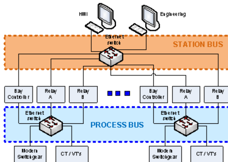
Figure 1 IEC 61850 Architecture
